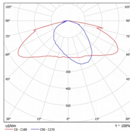
lens: socz-120x60
